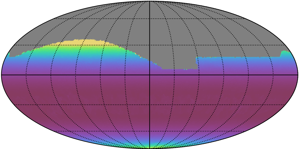
roll_uniform_early_half_accordion1_mjdp0_v3.4_10yrs All sky r band: Min airmass
