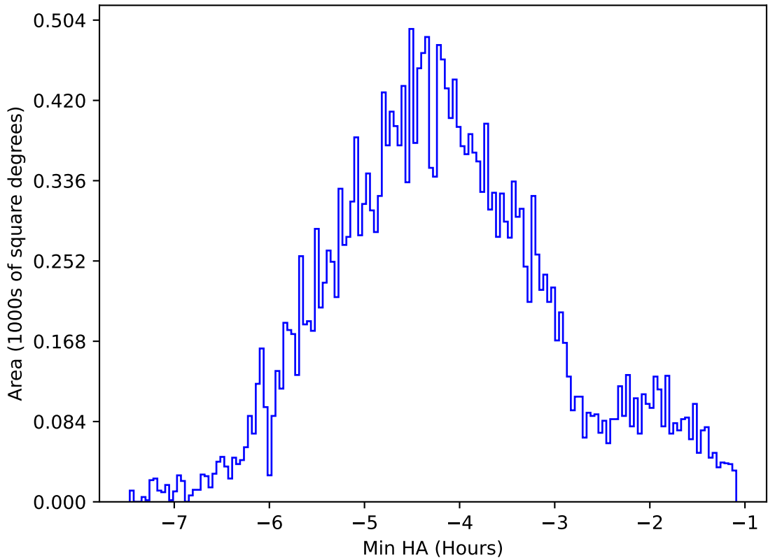
roll_uniform_early_half_accordion1_mjdp0_v3.4_10yrs All sky i band: Min HA
