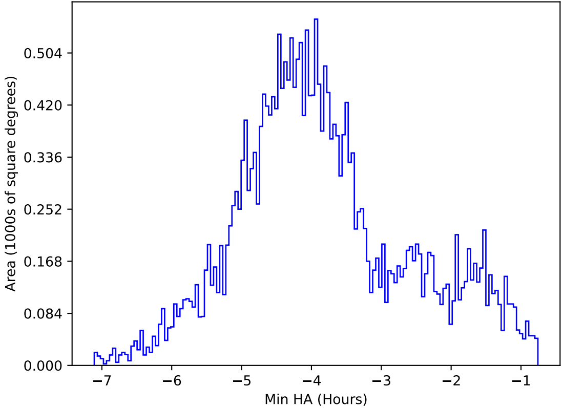
roll_uniform_early_half_accordion1_mjdp0_v3.4_10yrs All sky g band: Min HA
