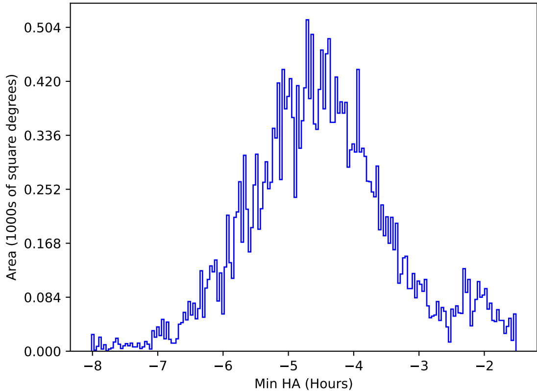
roll_uniform_early_half_accordion1_mjdp0_v3.4_10yrs All sky all bands: Min HA
