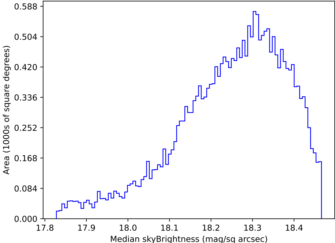
roll_uniform_early_half_accordion1_mjdp0_v3.4_10yrs Yr 1 y band: Median skyBrightness
