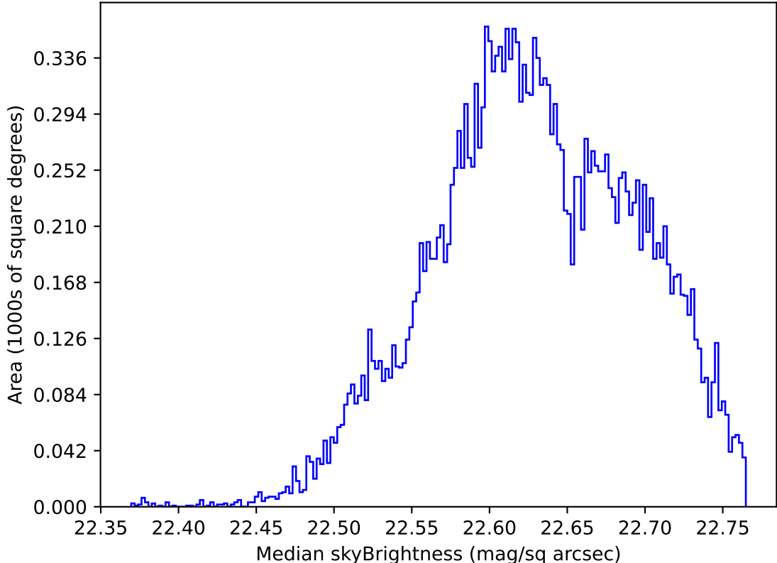
roll_uniform_early_half_accordion1_mjdp0_v3.4_10yrs Yr 1 u band: Median skyBrightness
