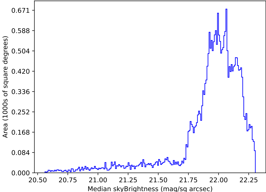
roll_uniform_early_half_accordion1_mjdp0_v3.4_10yrs Yr 1 g band: Median skyBrightness
