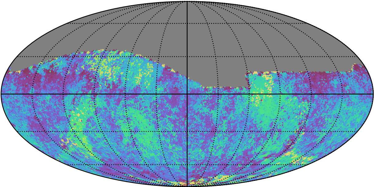
roll_uniform_early_half_accordion1_mjdp0_v3.4_10yrs Yr 1 all bands: Median skyBrightness
