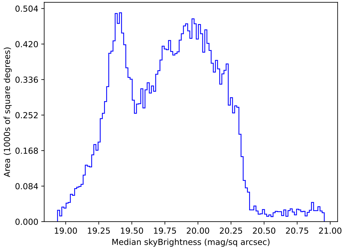
roll_uniform_early_half_accordion1_mjdp0_v3.4_10yrs Yr 1 all bands: Median skyBrightness
