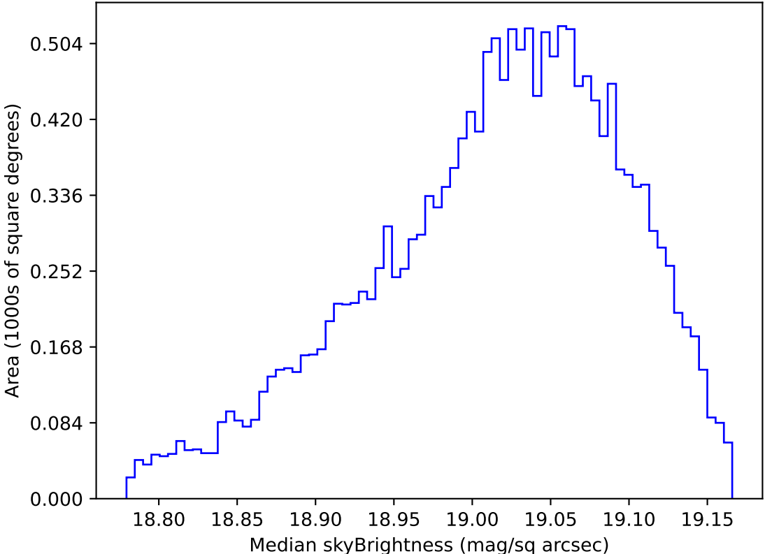
roll_uniform_early_half_accordion1_mjdp0_v3.4_10yrs WFD z band: Median skyBrightness
