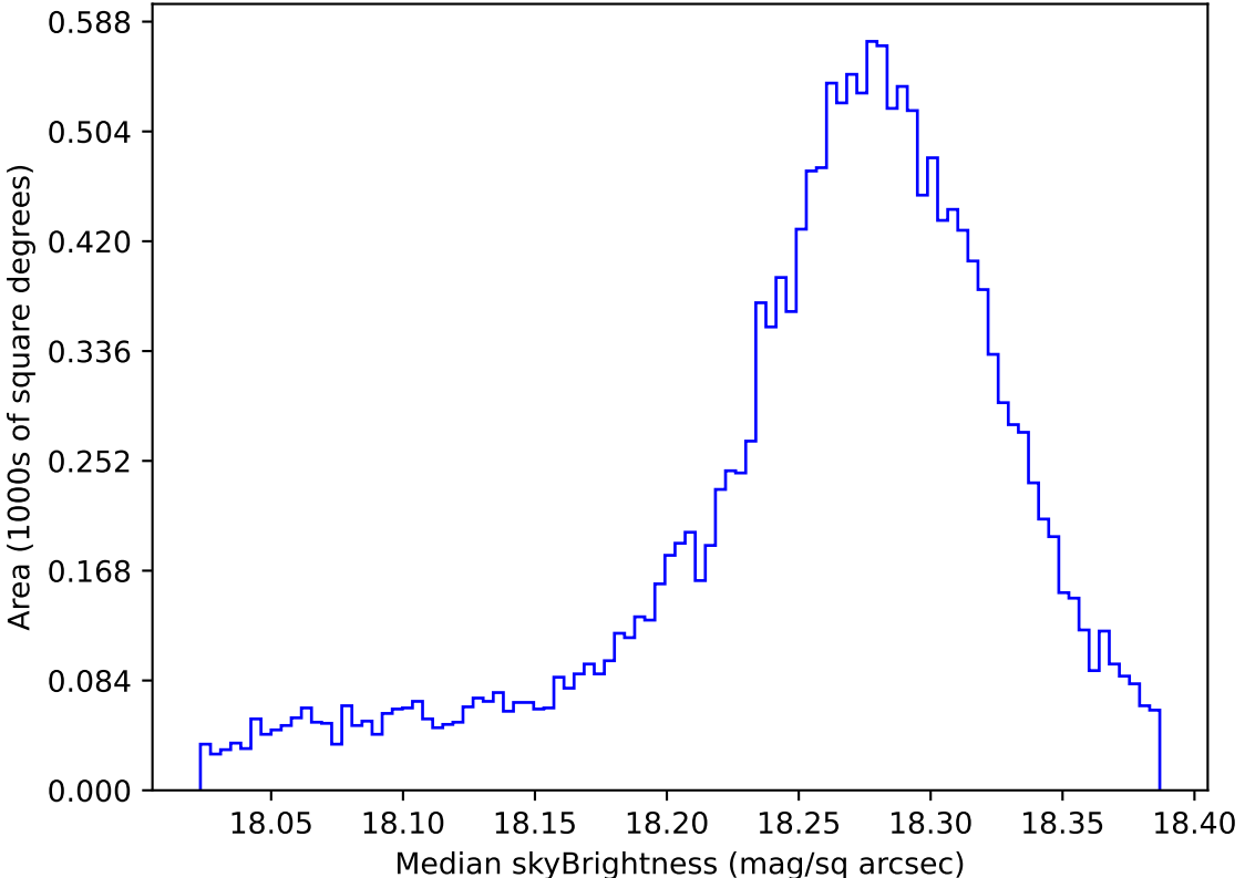
roll_uniform_early_half_accordion1_mjdp0_v3.4_10yrs WFD y band: Median skyBrightness
