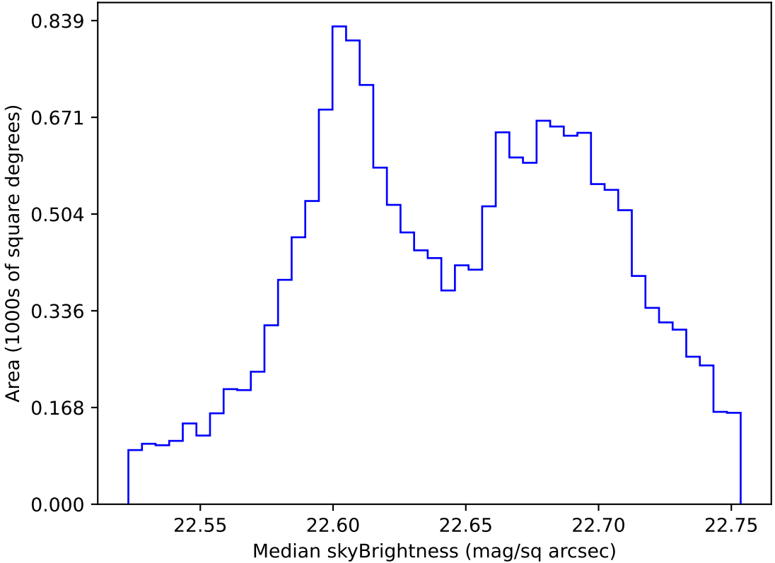
roll_uniform_early_half_accordion1_mjdp0_v3.4_10yrs WFD u band: Median skyBrightness
