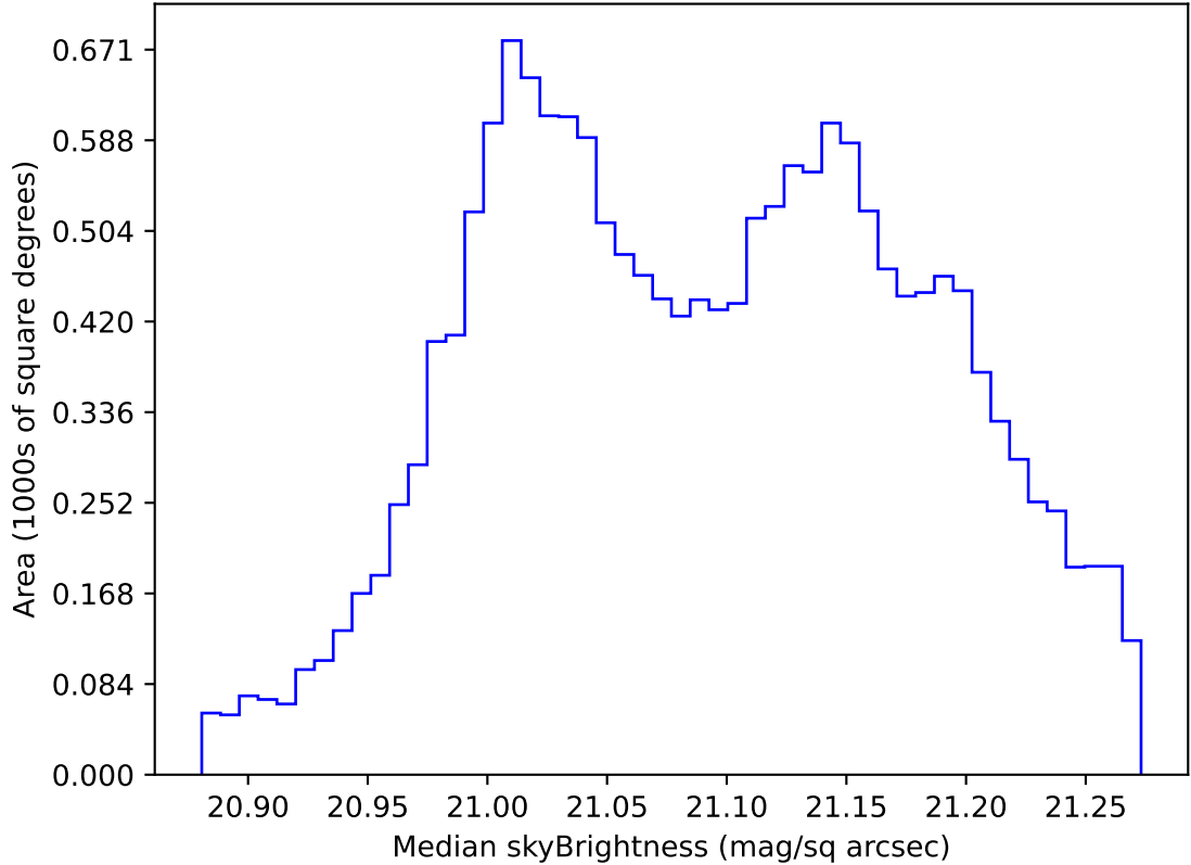
roll_uniform_early_half_accordion1_mjdp0_v3.4_10yrs WFD r band: Median skyBrightness
