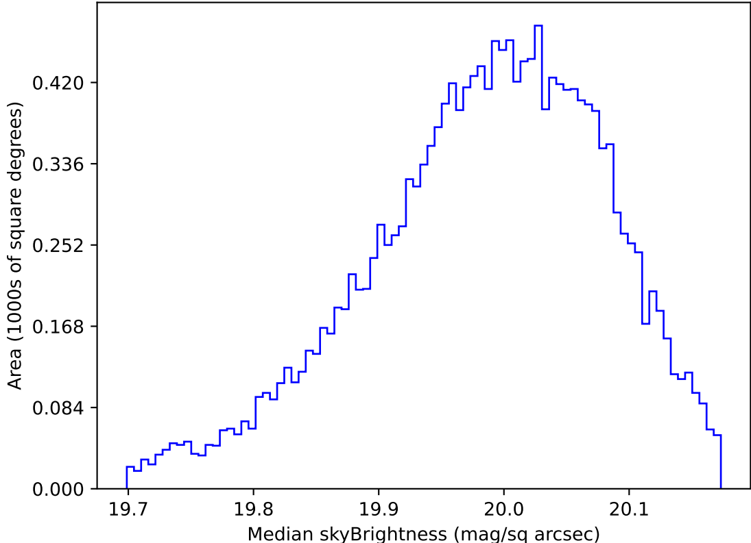
roll_uniform_early_half_accordion1_mjdp0_v3.4_10yrs WFD i band: Median skyBrightness
