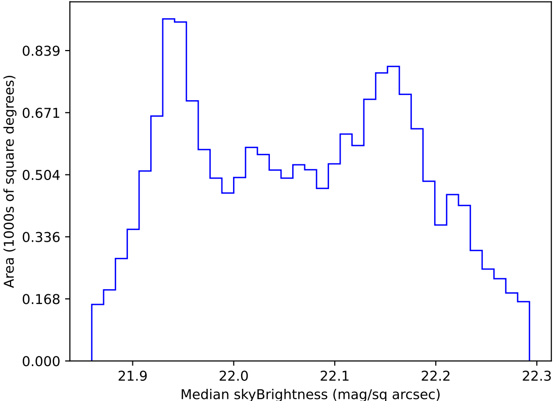
roll_uniform_early_half_accordion1_mjdp0_v3.4_10yrs WFD g band: Median skyBrightness
