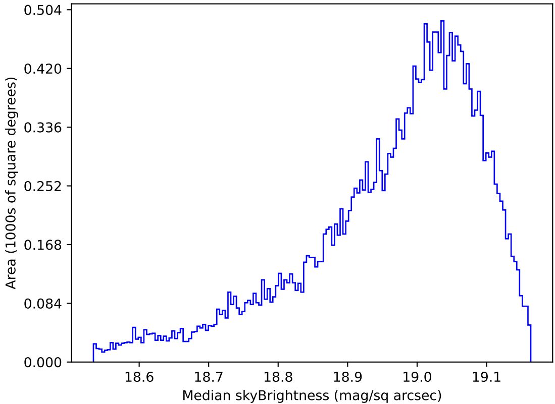
roll_uniform_early_half_accordion1_mjdp0_v3.4_10yrs All sky z band: Median skyBrightness
