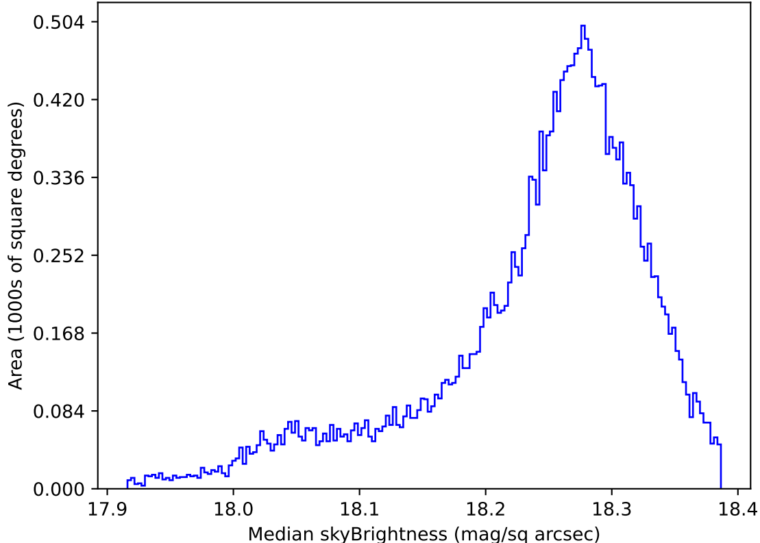
roll_uniform_early_half_accordion1_mjdp0_v3.4_10yrs All sky y band: Median skyBrightness
