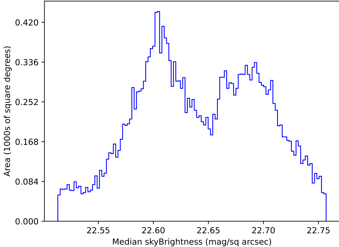
roll_uniform_early_half_accordion1_mjdp0_v3.4_10yrs All sky u band: Median skyBrightness
