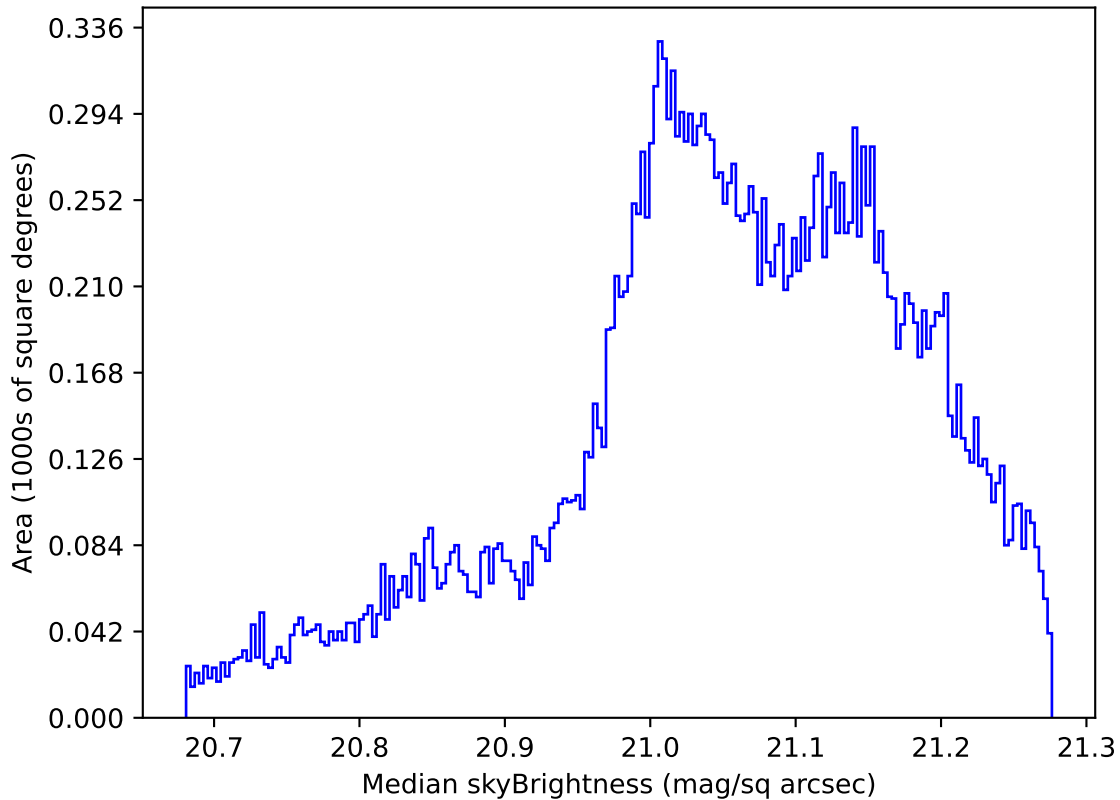
roll_uniform_early_half_accordion1_mjdp0_v3.4_10yrs All sky r band: Median skyBrightness
