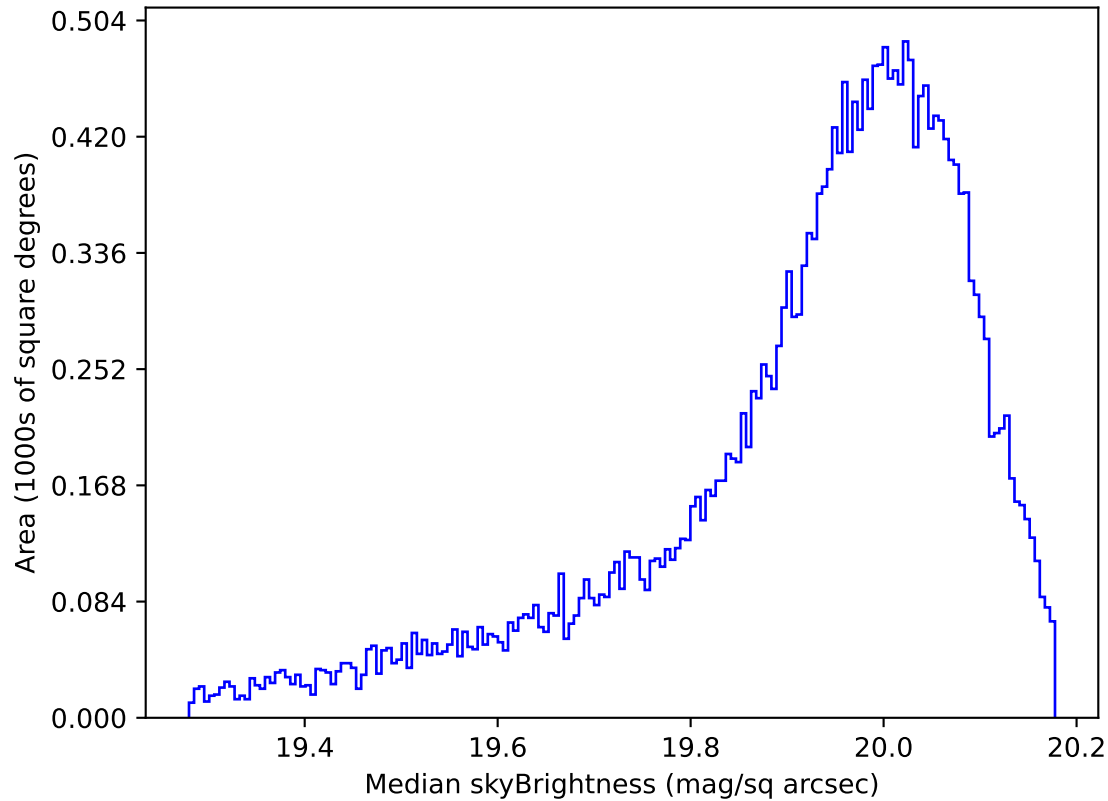
roll_uniform_early_half_accordion1_mjdp0_v3.4_10yrs All sky i band: Median skyBrightness
