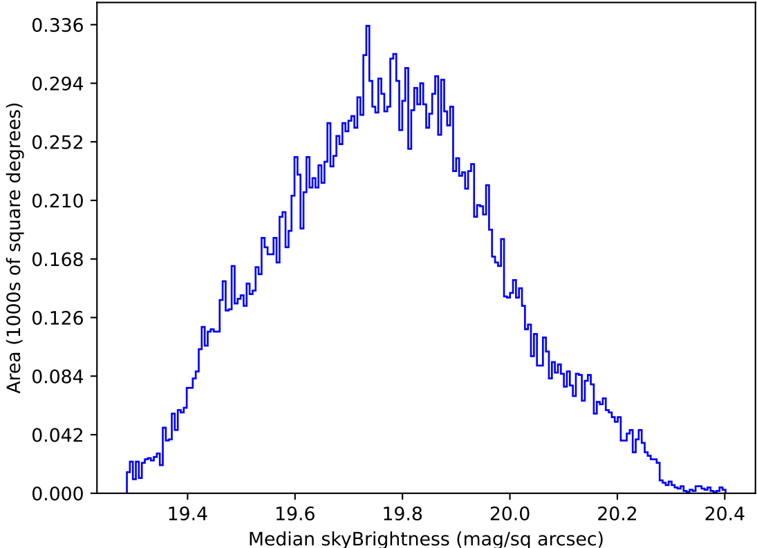
roll_uniform_early_half_accordion1_mjdp0_v3.4_10yrs All sky all bands: Median skyBrightness
