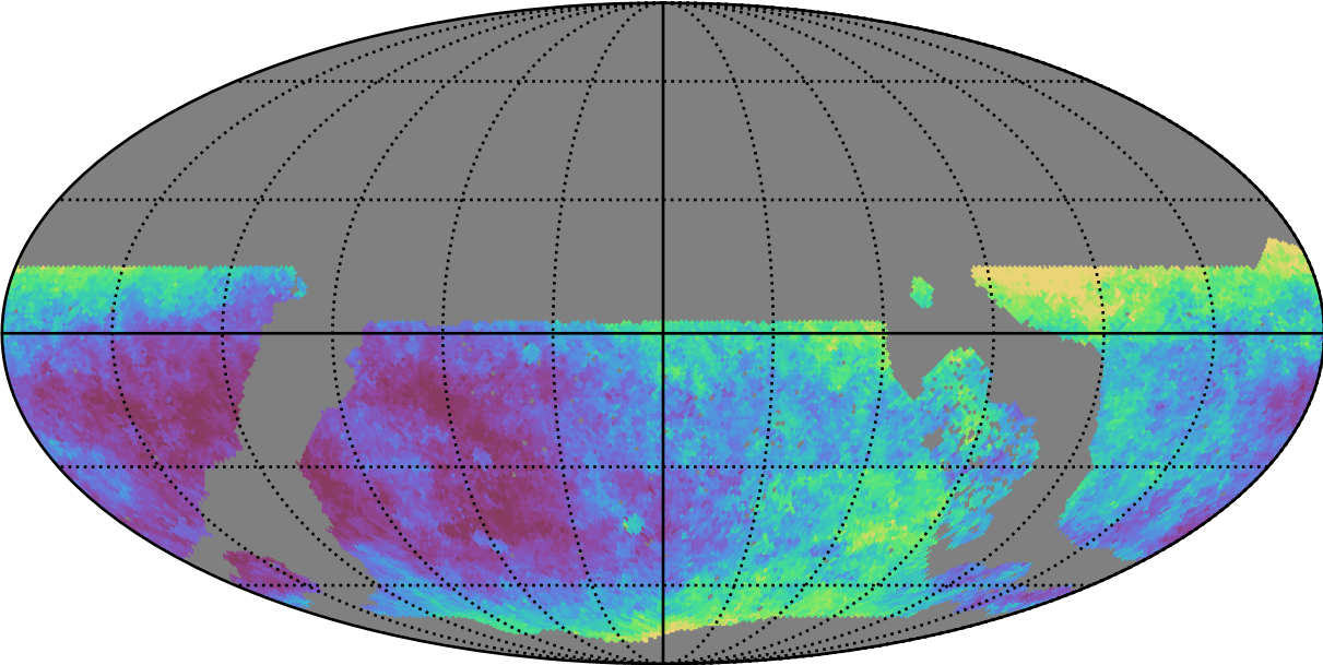
roll_uniform_early_half_accordion1_mjdp0_v3.4_10yrs WFD y band: Median seeingEff
