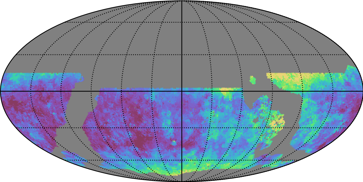
roll_uniform_early_half_accordion1_mjdp0_v3.4_10yrs WFD u band: Median seeingEff
