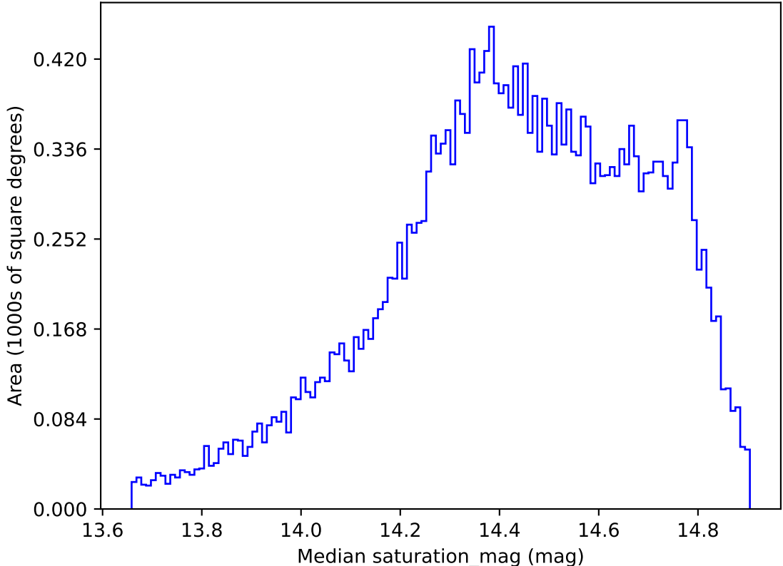
roll_uniform_early_half_accordion1_mjdp0_v3.4_10yrs All sky i band: Median saturation_mag
