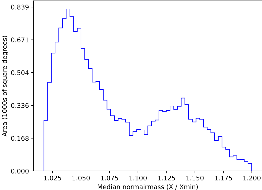
roll_uniform_early_half_accordion1_mjdp0_v3.4_10yrs WFD g band: Median normairmass
