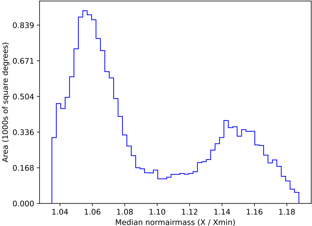
roll_uniform_early_half_accordion1_mjdp0_v3.4_10yrs WFD all bands: Median normairmass
