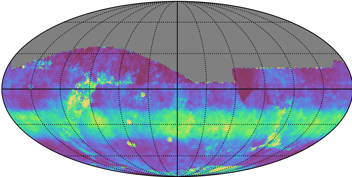
roll_uniform_early_half_accordion1_mjdp0_v3.4_10yrs All sky z band: Median normairmass
