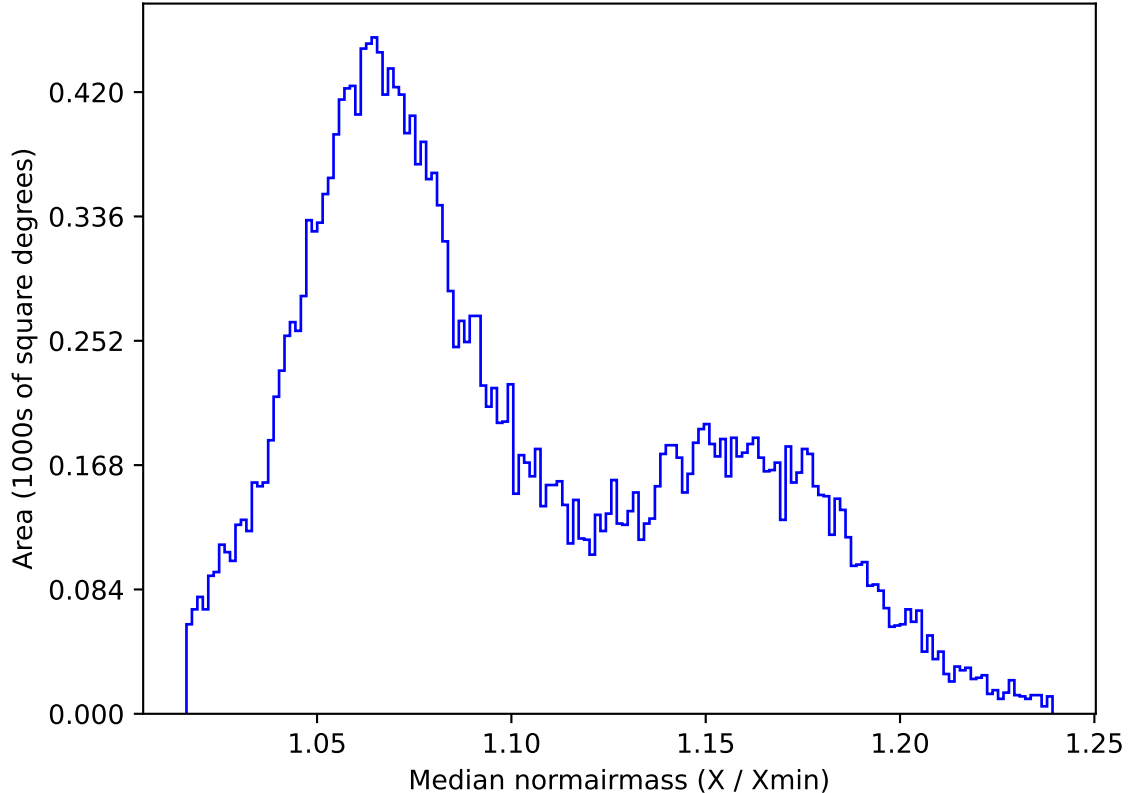
roll_uniform_early_half_accordion1_mjdp0_v3.4_10yrs All sky z band: Median normairmass
