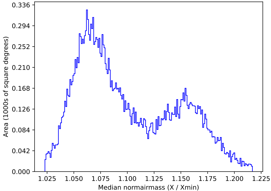
roll_uniform_early_half_accordion1_mjdp0_v3.4_10yrs All sky y band: Median normairmass
