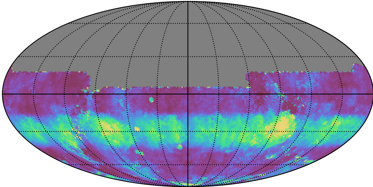
roll_uniform_early_half_accordion1_mjdp0_v3.4_10yrs All sky u band: Median normairmass
