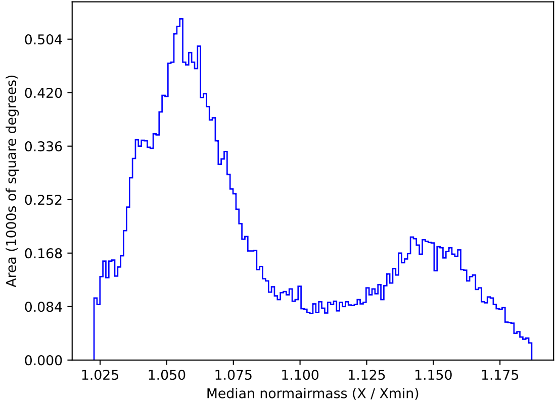
roll_uniform_early_half_accordion1_mjdp0_v3.4_10yrs All sky all bands: Median normairmass
