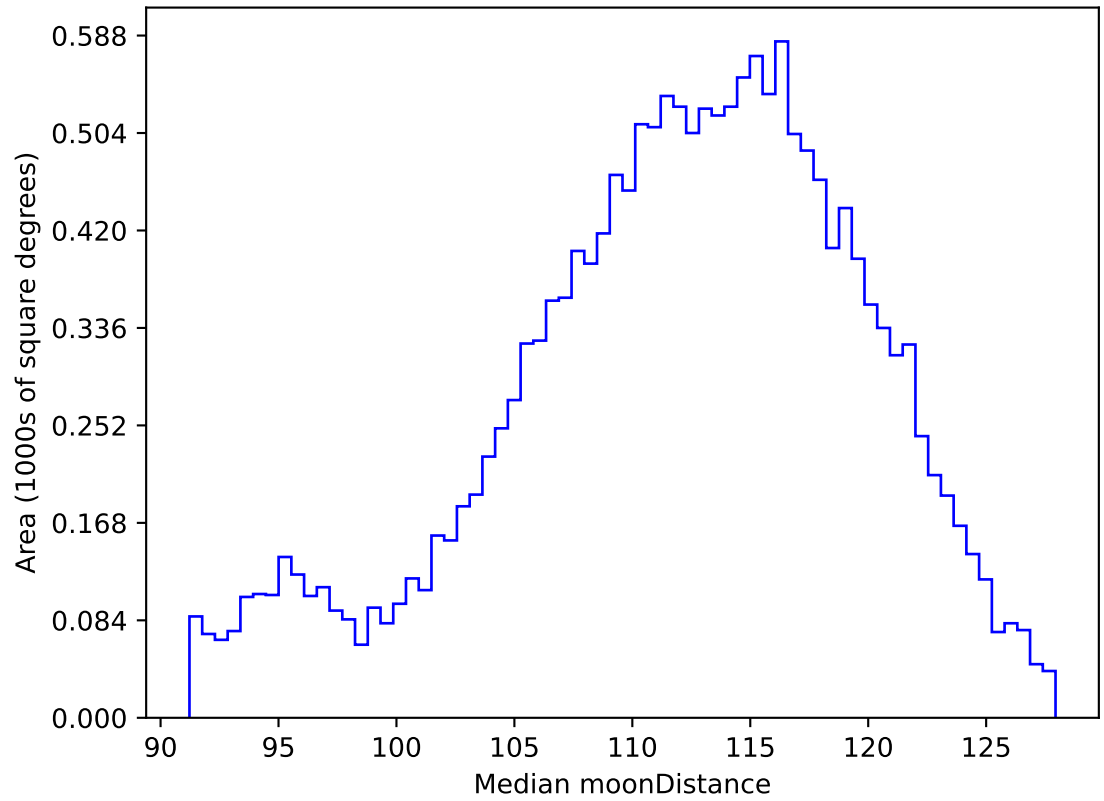
roll_uniform_early_half_accordion1_mjdp0_v3.4_10yrs WFD r band: Median moonDistance
