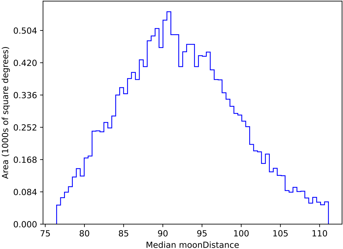
roll_uniform_early_half_accordion1_mjdp0_v3.4_10yrs WFD i band: Median moonDistance
