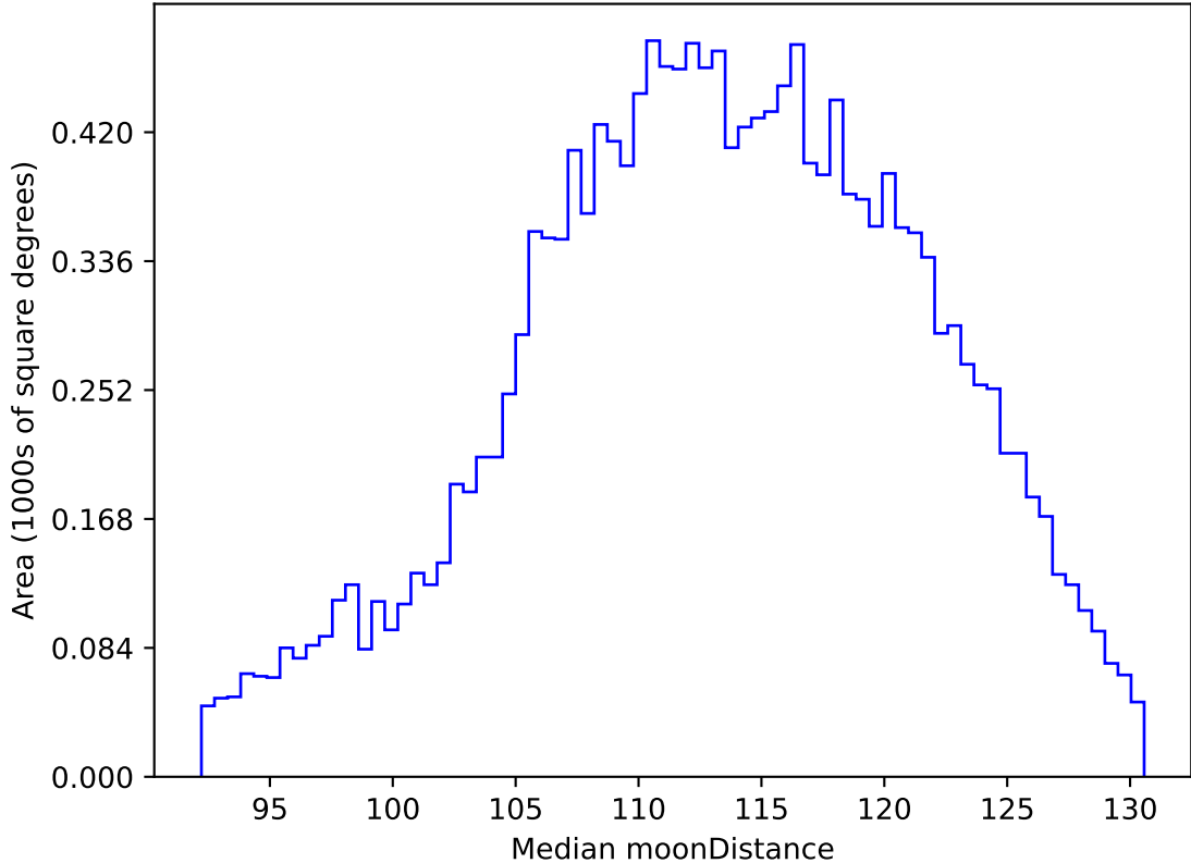
roll_uniform_early_half_accordion1_mjdp0_v3.4_10yrs WFD g band: Median moonDistance
