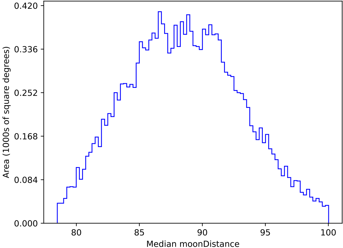
roll_uniform_early_half_accordion1_mjdp0_v3.4_10yrs WFD all bands: Median moonDistance
