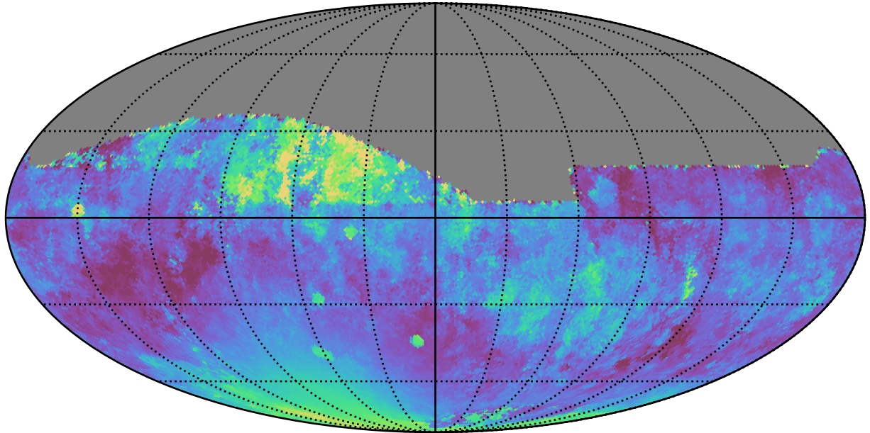
roll_uniform_early_half_accordion1_mjdp0_v3.4_10yrs All sky z band: Median moonDistance
