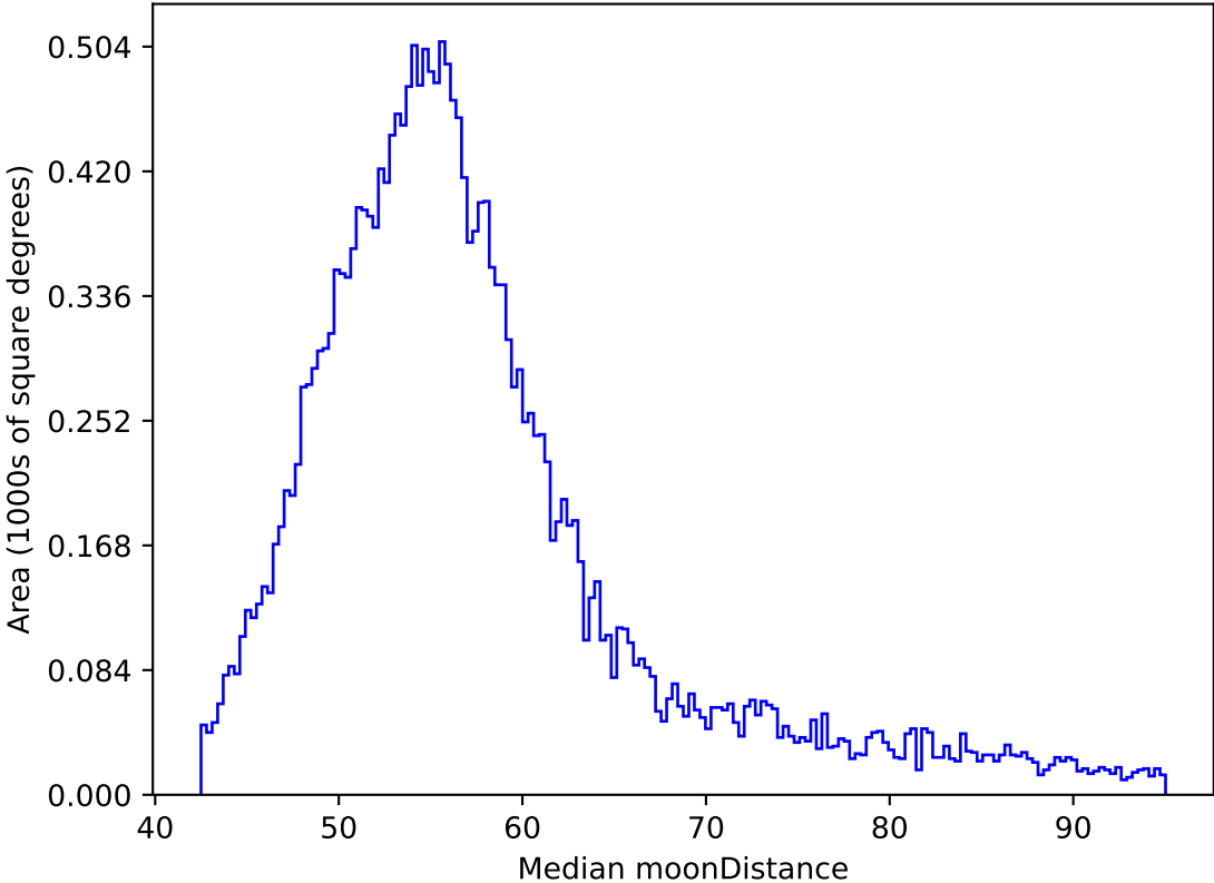
roll_uniform_early_half_accordion1_mjdp0_v3.4_10yrs All sky y band: Median moonDistance
