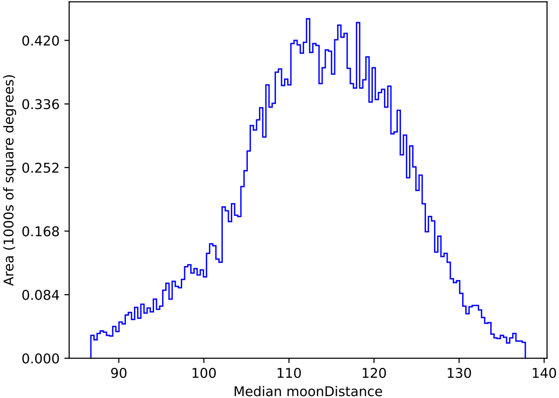
roll_uniform_early_half_accordion1_mjdp0_v3.4_10yrs All sky g band: Median moonDistance
