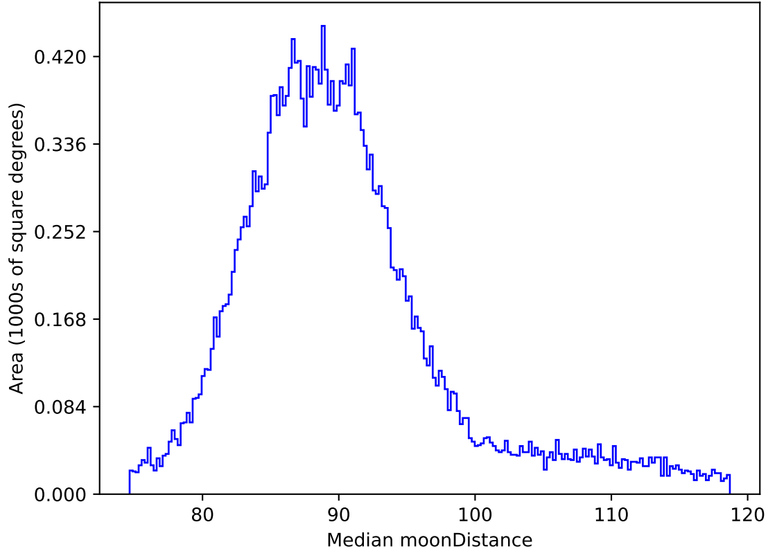
roll_uniform_early_half_accordion1_mjdp0_v3.4_10yrs All sky all bands: Median moonDistance
