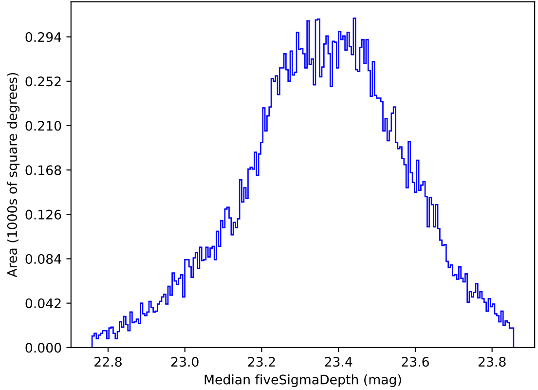
roll_uniform_early_half_accordion1_mjdp0_v3.4_10yrs Yr 1 all bands: Median fiveSigmaDepth
