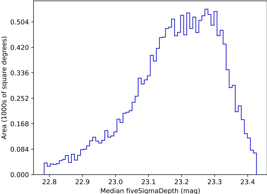
roll_uniform_early_half_accordion1_mjdp0_v3.4_10yrs WFD u band: Median fiveSigmaDepth
