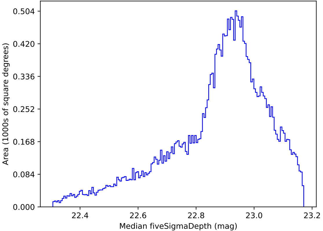
roll_uniform_early_half_accordion1_mjdp0_v3.4_10yrs All sky z band: Median fiveSigmaDepth
