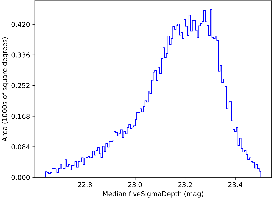
roll_uniform_early_half_accordion1_mjdp0_v3.4_10yrs All sky u band: Median fiveSigmaDepth
