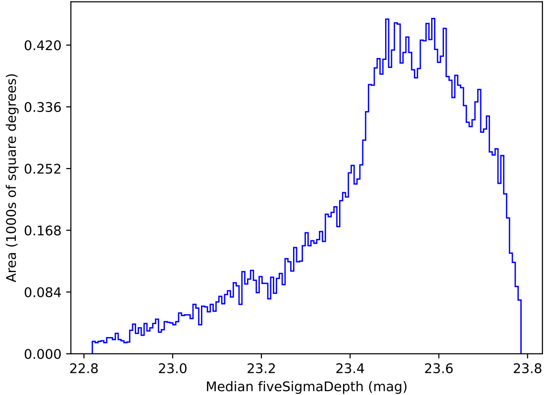
roll_uniform_early_half_accordion1_mjdp0_v3.4_10yrs All sky i band: Median fiveSigmaDepth
