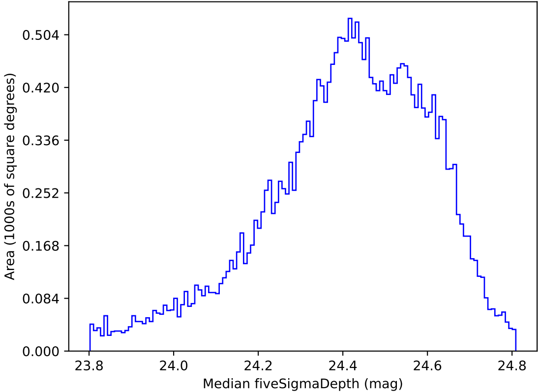
roll_uniform_early_half_accordion1_mjdp0_v3.4_10yrs All sky g band: Median fiveSigmaDepth
