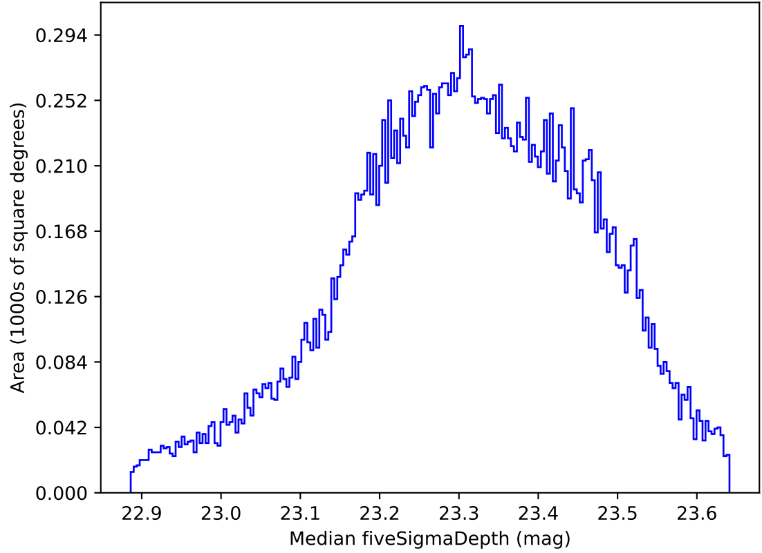
roll_uniform_early_half_accordion1_mjdp0_v3.4_10yrs All sky all bands: Median fiveSigmaDepth
