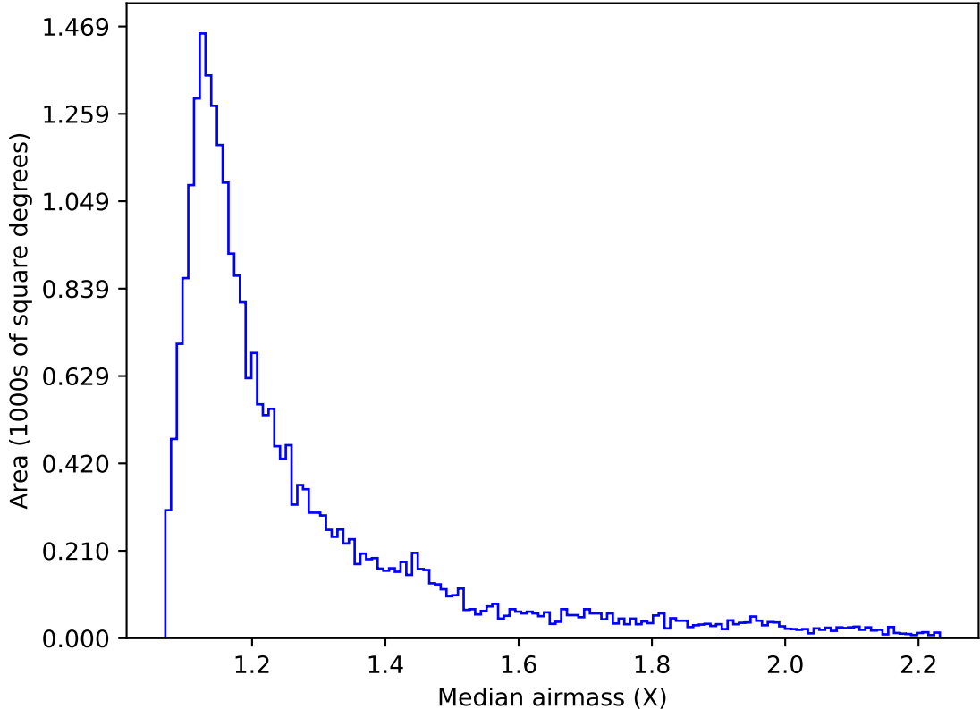
roll_uniform_early_half_accordion1_mjdp0_v3.4_10yrs Yr 1 z band: Median airmass
