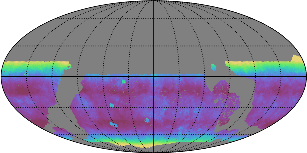
roll_uniform_early_half_accordion1_mjdp0_v3.4_10yrs WFD z band: Median airmass
