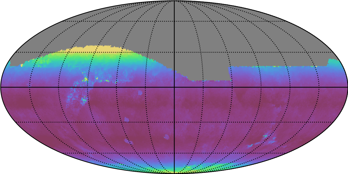
roll_uniform_early_half_accordion1_mjdp0_v3.4_10yrs All sky z band: Median airmass
