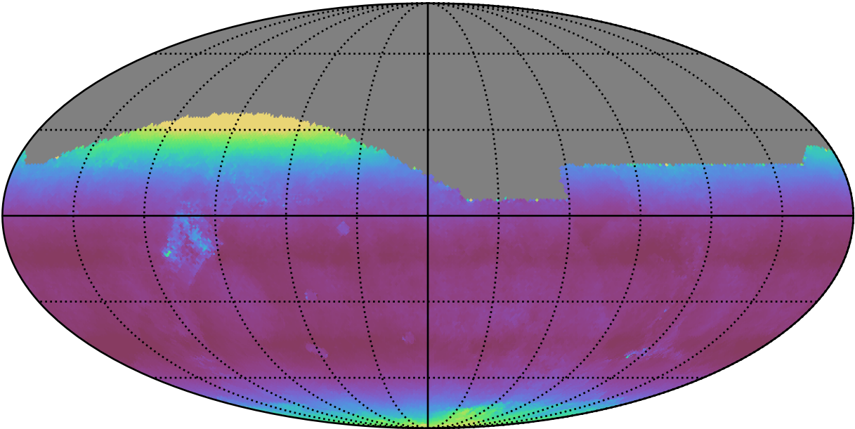
roll_uniform_early_half_accordion1_mjdp0_v3.4_10yrs All sky i band: Median airmass
